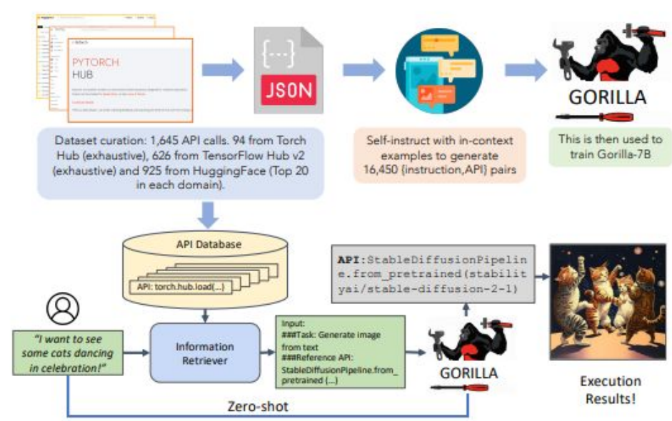
Figure 3: Gorilla: A system for enabling LLMs to interact with APIs. The upper half represents the training procedure as described in Sec 3. This is the most exhaustive API data-set for ML to the best of our knowledge. During inference (lower half), Gorilla supports two modes - with retrieval, and zero-shot. In this example, it is able to suggest the right API call for generating the image from the user's natural language query.
